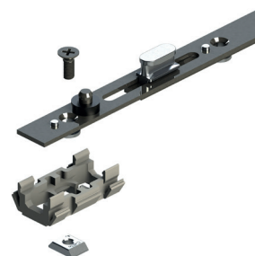
Expansion fixing (A2)
