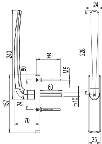
PRIMA window handle dimensions L240 -I80
