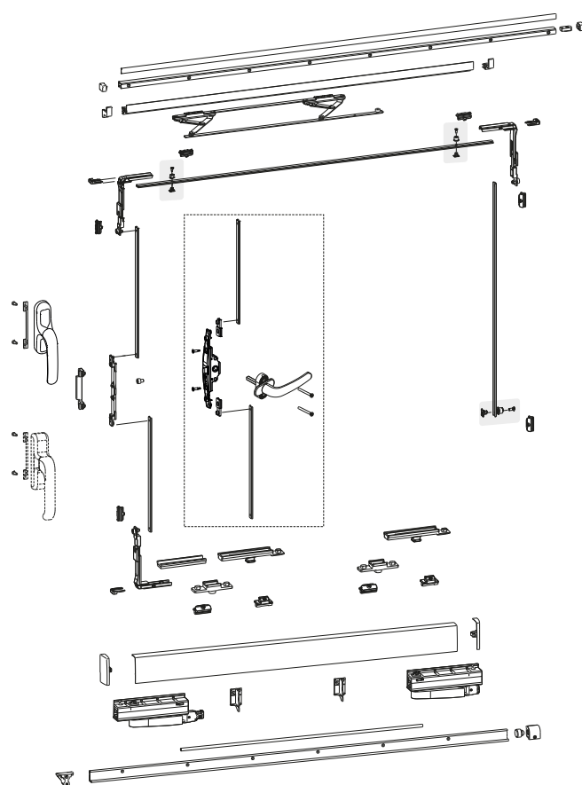
Scheme for GS1000-ML R40 profile with cremone/window handle
