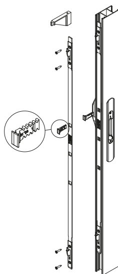
Version A: Connection to nib
