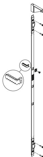
Version B: Connection to nib screwed in
