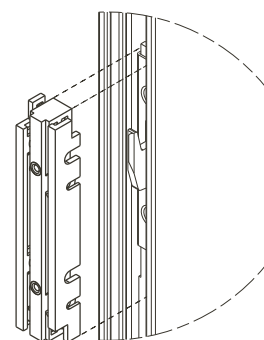
Centring template
